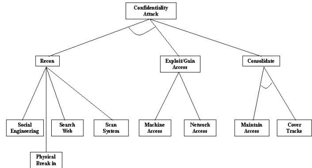
Figure 5: Example Confidentiality Attack Tree
